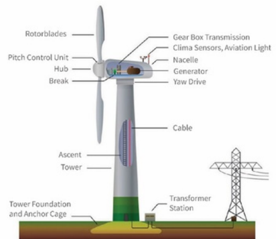
Wind turbine components. Source: powerandbeyond.com, 2024
